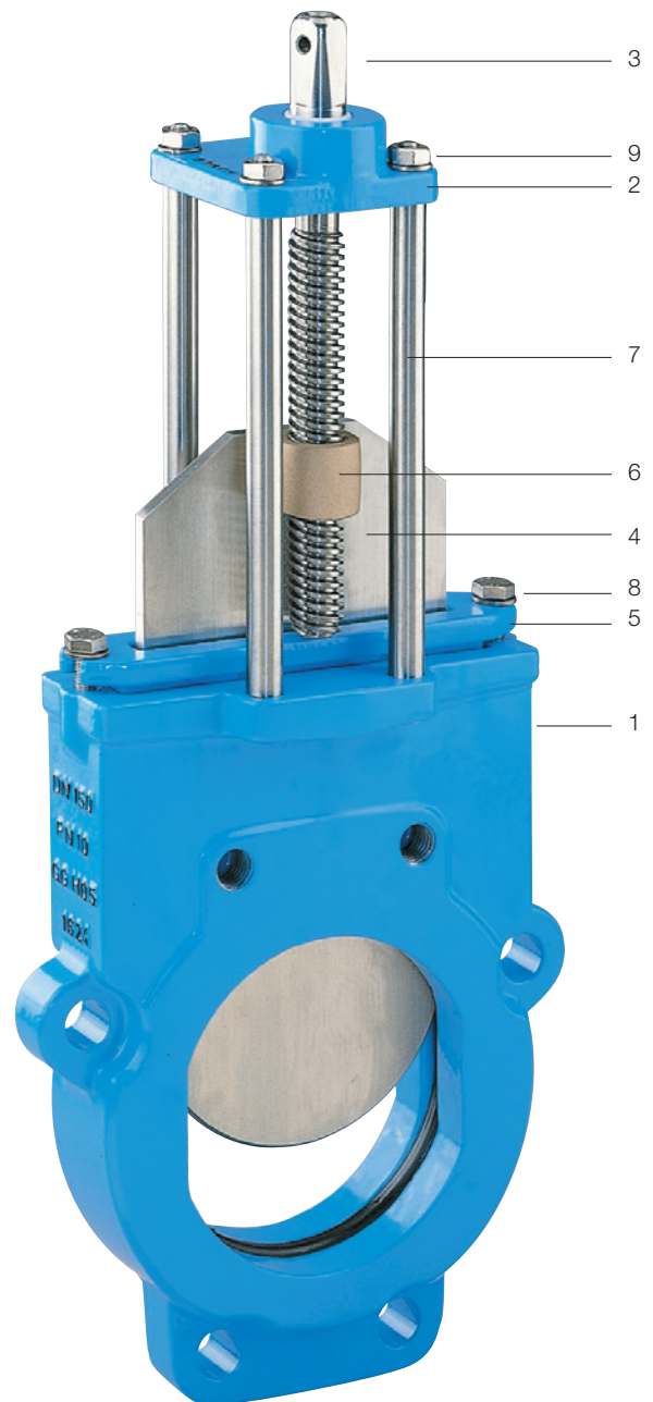
illustration DN 50 - 200
